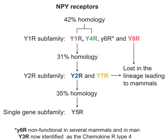
FIGURE 3: NPY receptors. Y 1 R, Y 2 R, Y 4 R and Y 5 R are the four active receptors in mammals. y 6 R is functionally inactive and Y 7 R and Y 8 R got lost in the lineage leading to mammals.
