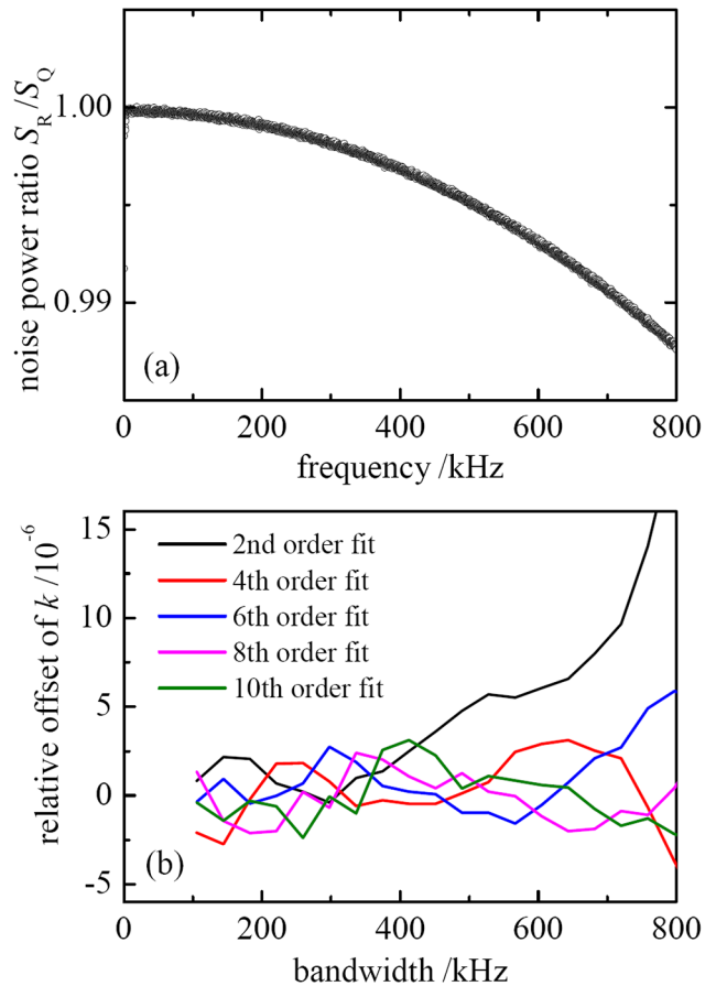
Figure 7. (a) The noise power ratio spectrum from the NIM 2017 measurements, where S_R and S_Q are the measured power spectral densities of thermal noise and quantum voltage noise, respectively, and (b) the estimate of relative offset of k from CODATA recommended value versus bandwidth and order of the even-order polynomial fit.
