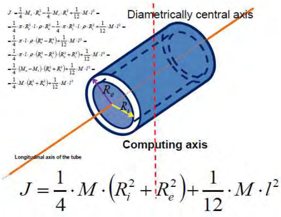
Fig. 11. Mass moment of inertia to a tube (pipe or annulus) determined about the diametrically central axis
