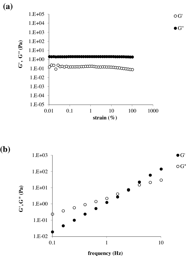
Fig. 4. Results of oscillatory measurements. (a) Dynamic moduli as a function of strain at 0.1 \text{ s}^{-1} frequency and (b) dynamic moduli as a function of frequency at constant strain (0.045%) for HA500/mucin mixtures. Measurements were performed at 35^\circ\text{C} . The trends shown are representative of all mixtures mucine/(selected HA sample).
