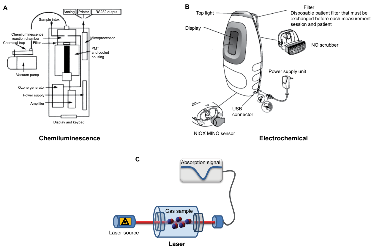
Figure 1 Schematic representation of a chemiluminescent analyzer (model 280i; Sievers) ( A ), an electrochemical sensor (NIOX MINO) ( B ), and a laser-based sensor ( C ). Abbreviations: NO, nitric oxide; PMT, photomultiplier tube.
